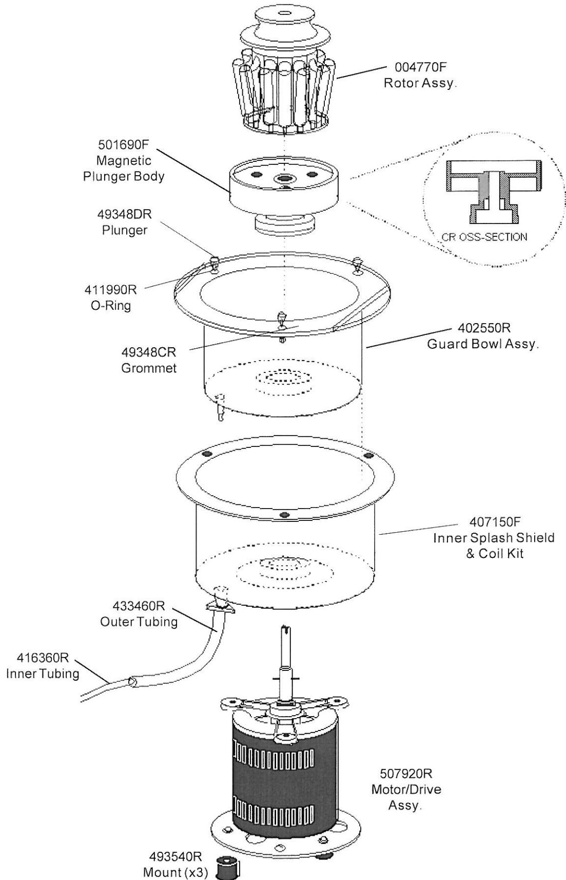
Figure 13-3 Drive Assembly
