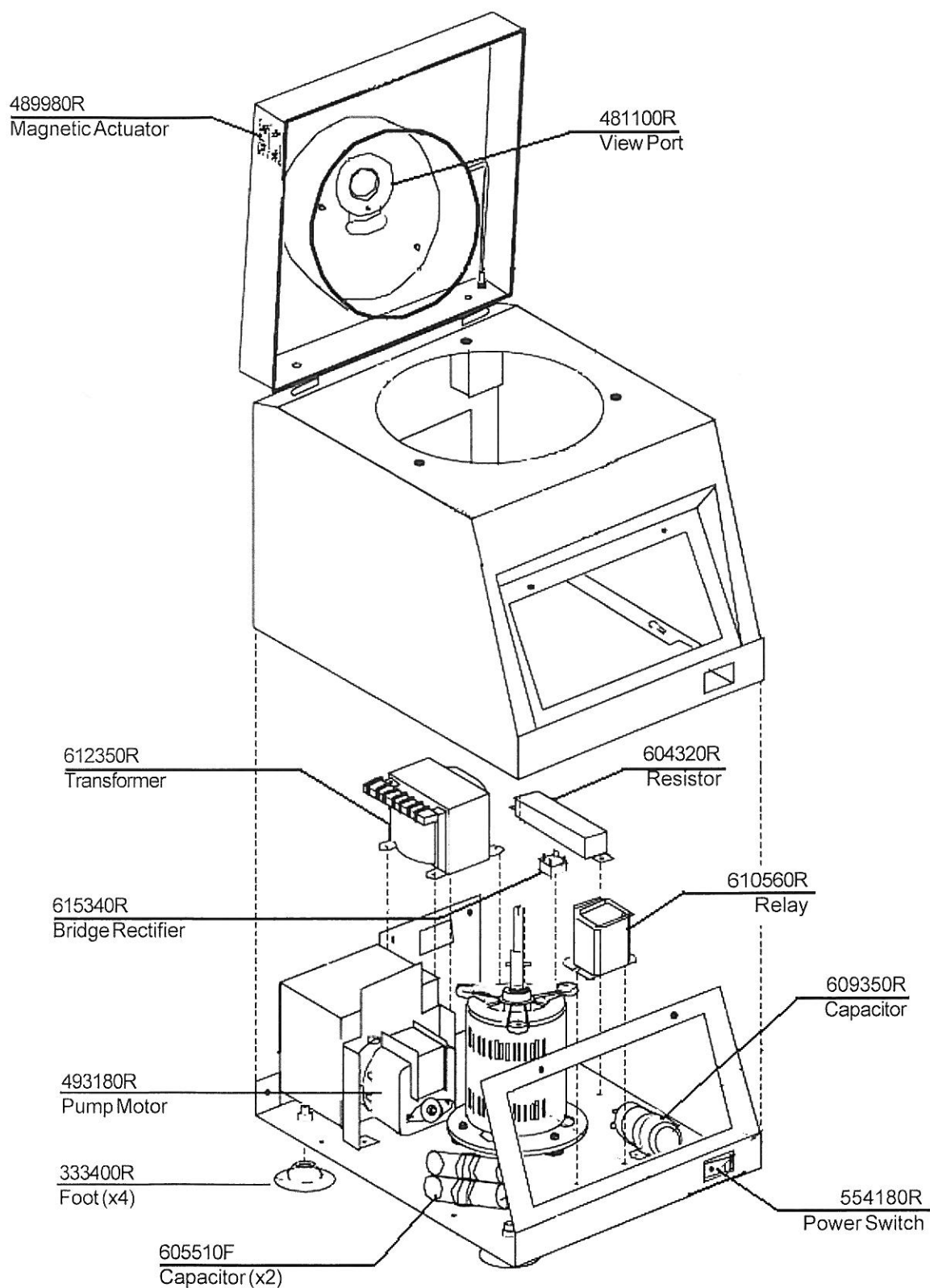
Figure 13-2 Base Assembly
