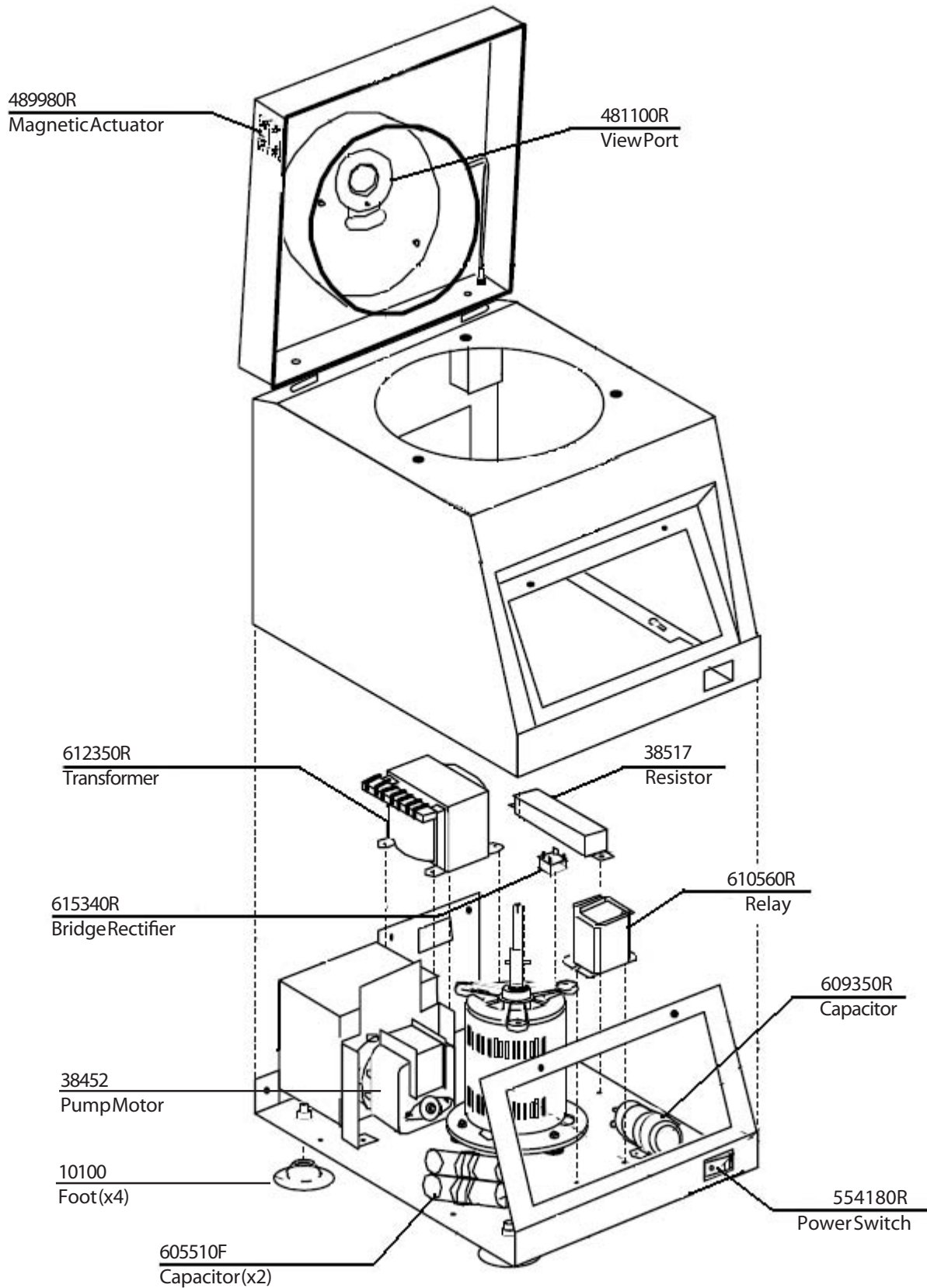
Figure 13-2 Base Assembly
