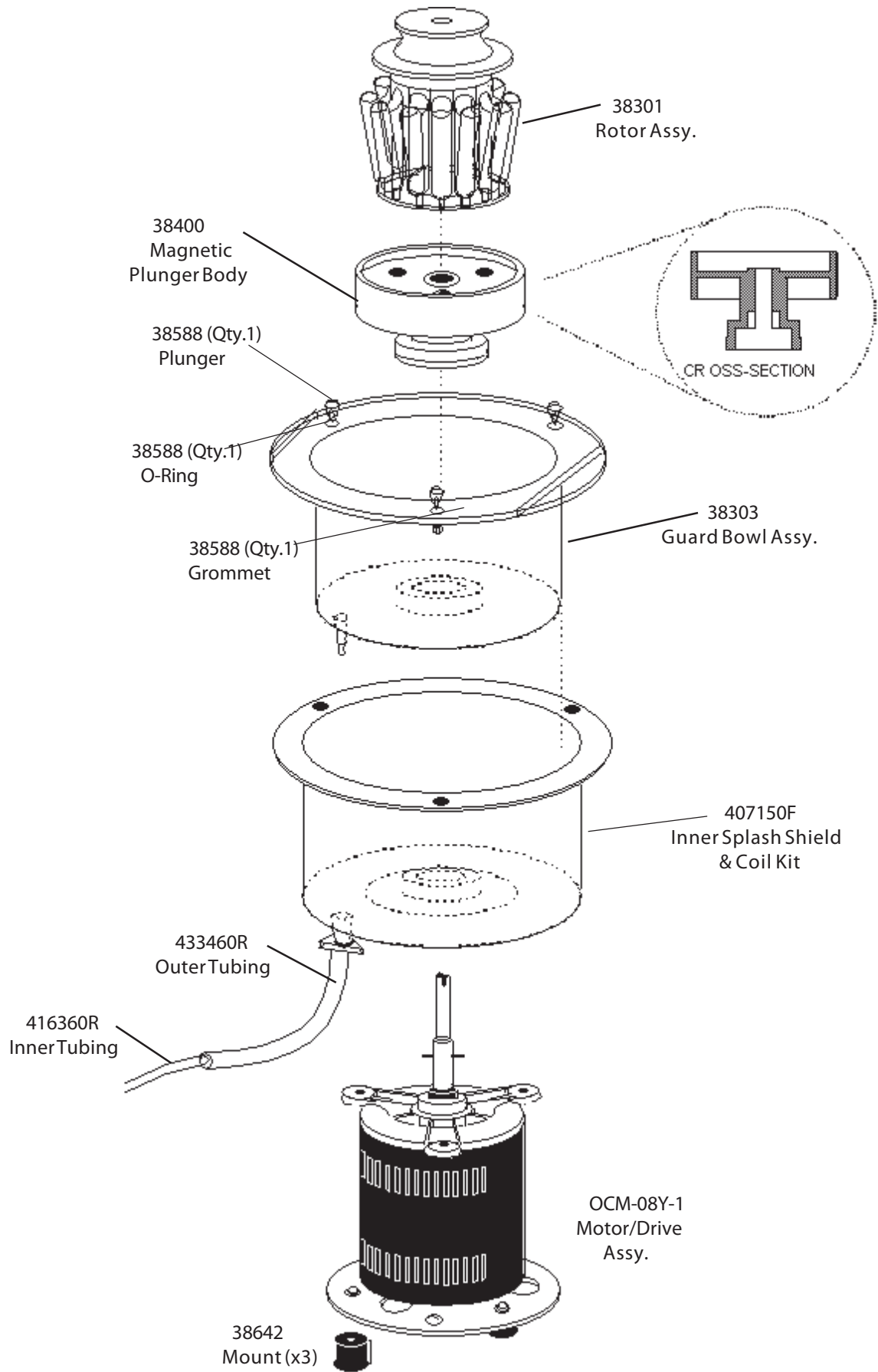
Figure 13-3 Drive Assembly
